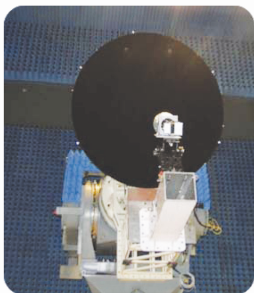
Figure 7. HGA in high power testing.
