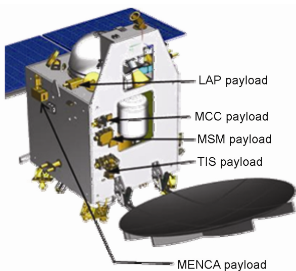
Figure 8. Payloads of MOM.
