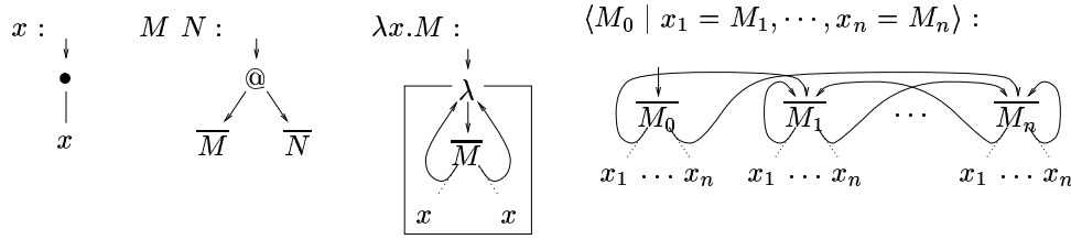
Figure 12. Pictorial definition of \rho_{\text{pre}}
