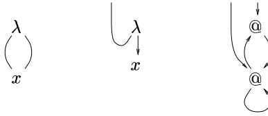
Figure 6. Examples of ill-formed lambda-graphs
