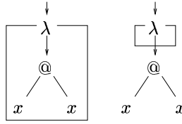
Figure 27. Two scoped graphs without an intermediate graph
