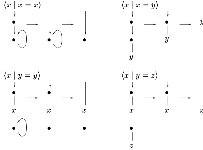
Figure 16. How simplification works with only variables
