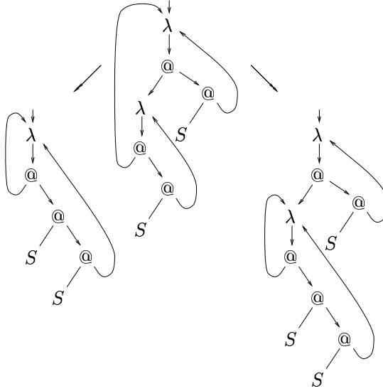
Figure 35. Failure of confluence of \lambda \circ
