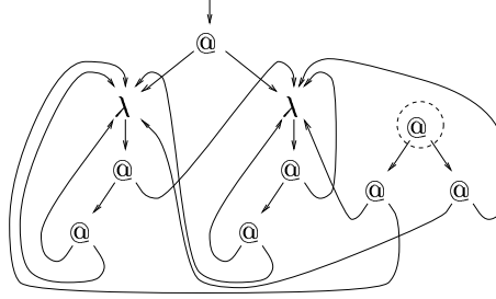
Figure 9. Example of ill-formed lambda-graph
