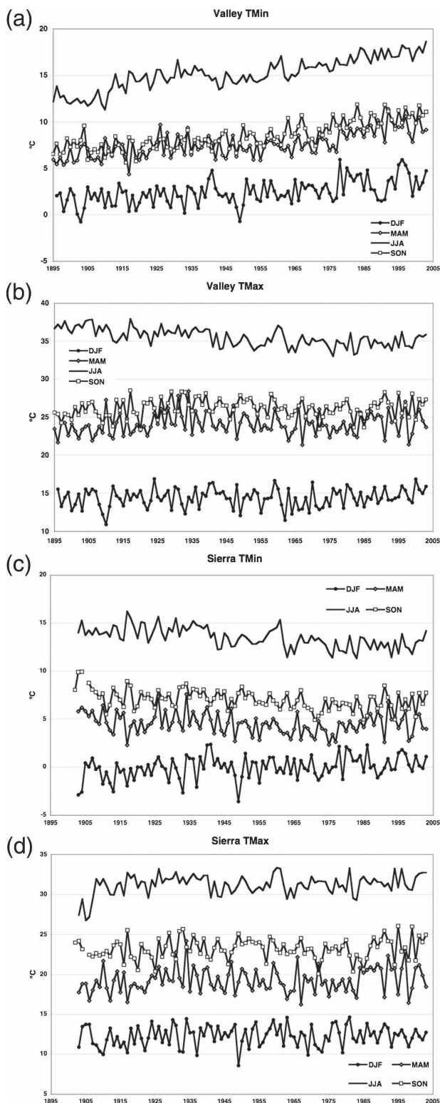
FIG. 7. (a)–(d) Time series of seasonal anomalies of Valley and Sierra TMin and TMax through 2003. (e) Time series of annual anomalies of mean temperature for Valley and Sierra stations.
