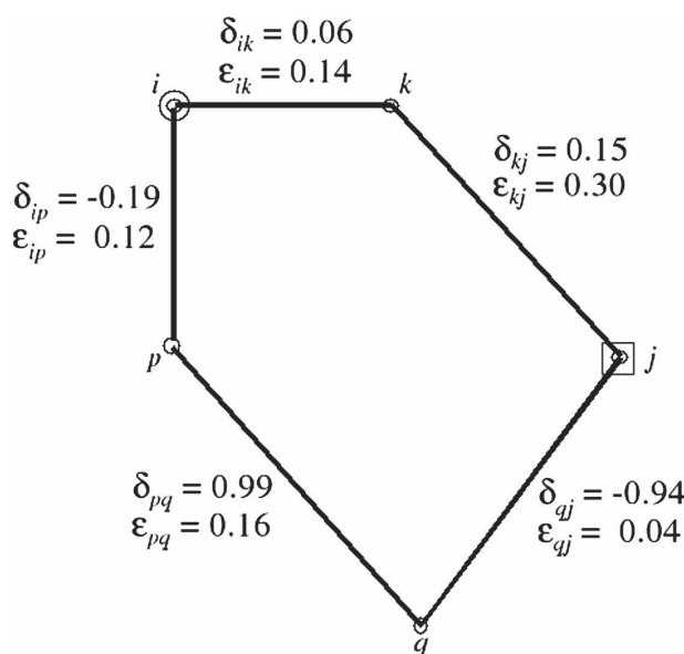
FIG. 6. A directed graph with vertices i, j, k, p , and q . There are two paths from vertex i , marked with an open circle, and vertex j , marked with an open square. One is through vertex k ; the other through vertices p and q . The edges of the graph are labeled with the bias ( \delta ) and the standard error ( \epsilon ). Using the definitions and conventions of Eqs. (1)–(3), we determine that the standard error of the path through vertex k is 0.33, whereas the standard error of the path through vertices p and q is 0.20. Hence, the least path from vertex i to vertex j is the one through vertices p and q , and we take the bias between vertices i and j to be the sum of the biases along the path through p and q , which is -0.14 . For simplicity, we have not shown the edges but assume that when the direction of traversal between two vertices changes, the algebraic sign of \delta is reversed.
