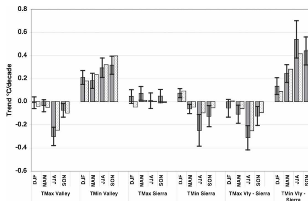
FIG. 8. Seasonal trends for each time series of Figs. 7a–d and trends of the difference time series. Solid gray bars represent trends from the original, full-segment calculations with error bars deduced from the combination of the 30-segment jackknife method and temporal sampling error. The lightly hashed bars represent the median trends of the nonparametric experiments.
